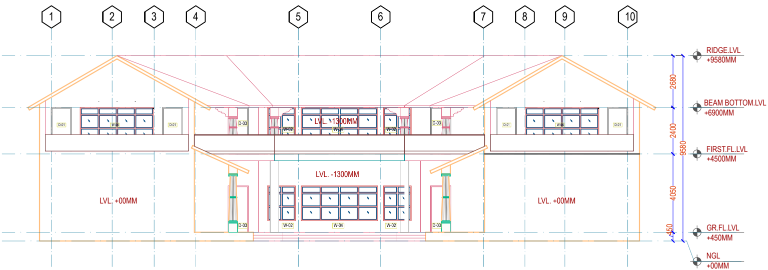
FRONT ELEVATION
